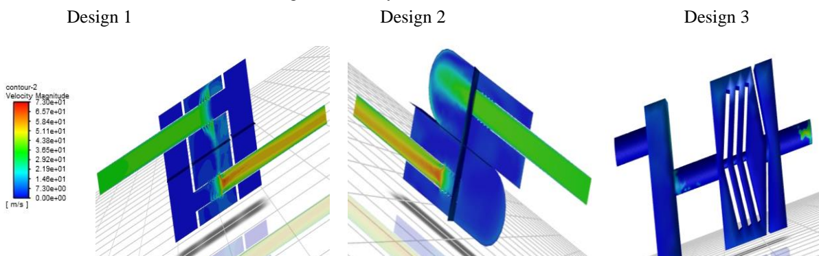
Fig. 7 - Velocity Contour of Muffler
