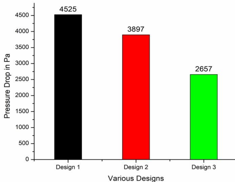
Fig. 10 - Pressure Drop across the model
