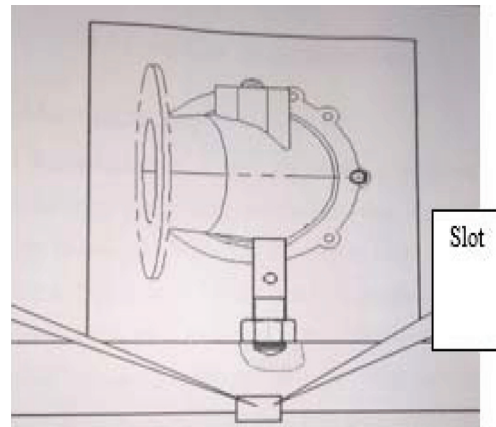
FIGURE 11. 2D Side view of the fixture
