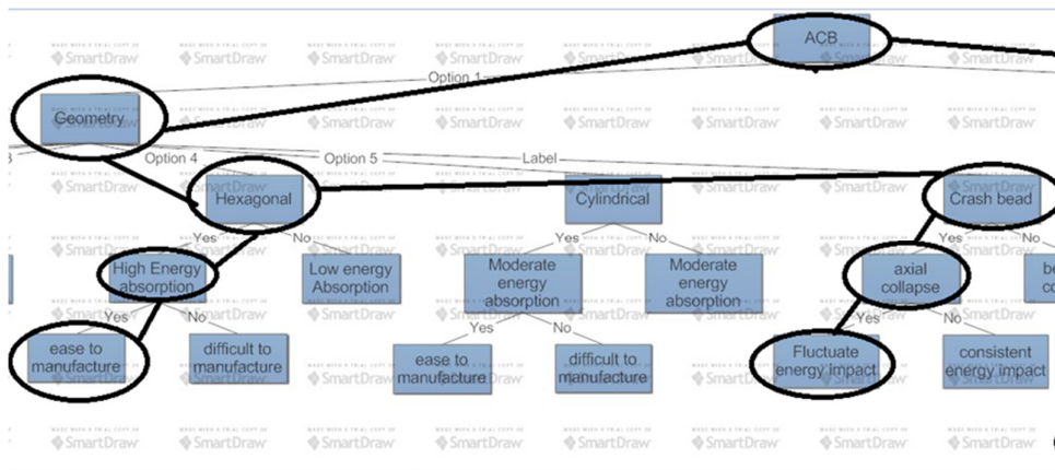
Fig. 5. Close up solution decision for requirements 1 (geometry)
