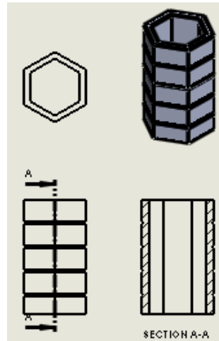
Fig. 7. ACB Conceptual Design
