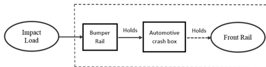
Fig.1. FAD for automotive crash box
