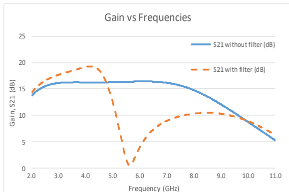
Figure 5: Effect of Notch Filter towards gain, S_{21} .
