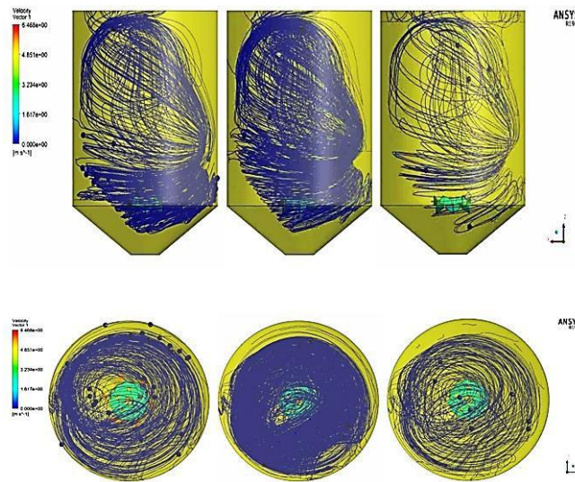
Fig 8 Velocity streamline results of improved mixer design.
